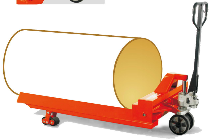
"Reel Carrying Truck" designed for carrying horizontal transport loads such as rolls, reels, cable drums etc.
